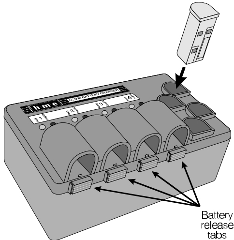
Figure 8. AC900 battery release tabs and battery going into storage port
